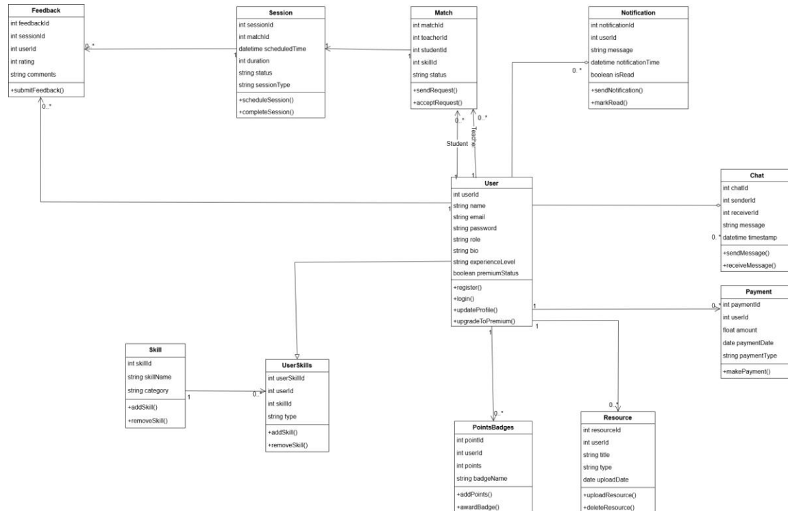
Figure 1: Class Diagram
